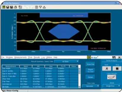
► XAUI compliance testing.
