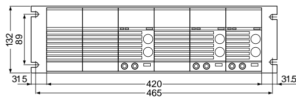
■ RACK for PS series RK-600E (EIA)
