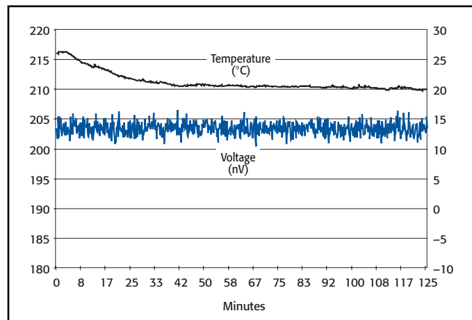
Figure 5. The Model 2182A's delta mode provides extremely stable results, even in the presence of large ambient temperature changes. In this challenging example, the 200nV signal results from a 20 \mu A current sourced by a model 6221 through a 10m \Omega test resistor.
