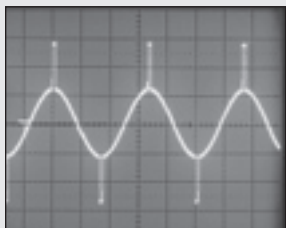
Sine wave with spikes from 85° - 95° and 265° - 275°
