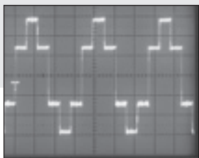
Six step sine wave
