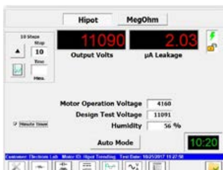
DC Hipot test screen with MINI controlling a Power Pack
