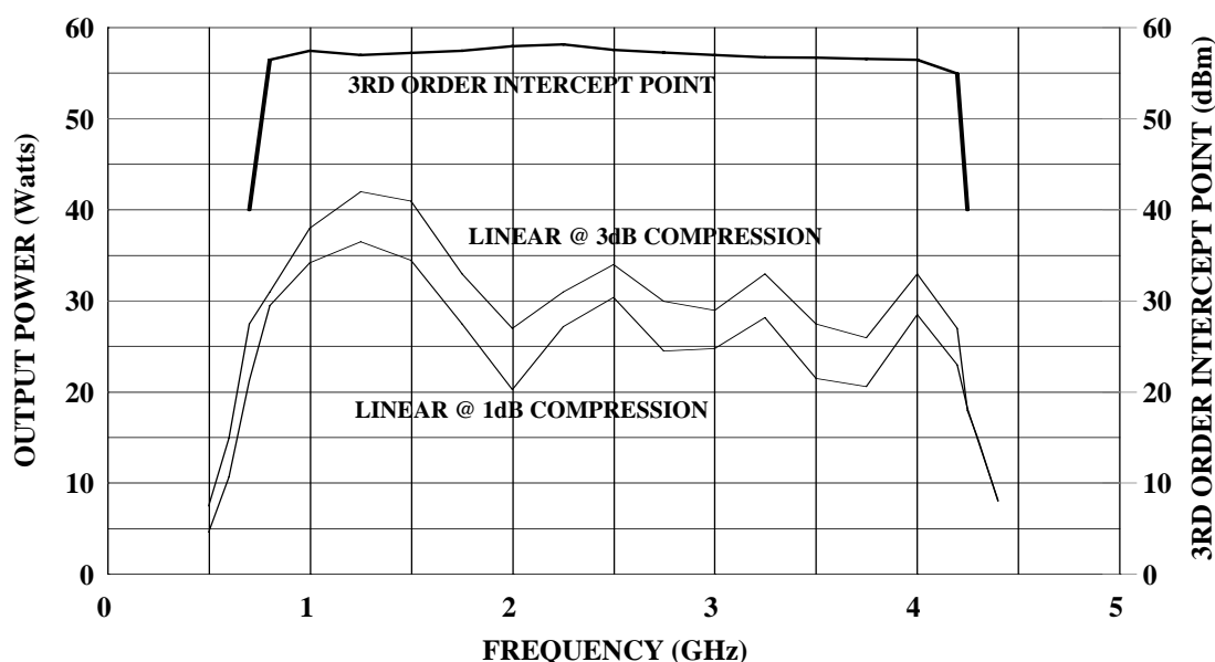
25S1G4A Typical Performance
