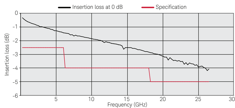
Figure 4. Keysight J7211A attenuation control unit insertion loss (at 0 dB) versus frequency
