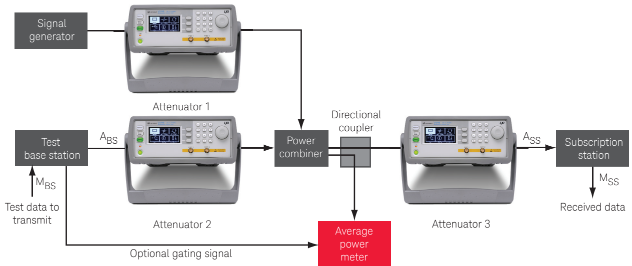
Figure 3. Test setup for 1 st adjacent channel interference
