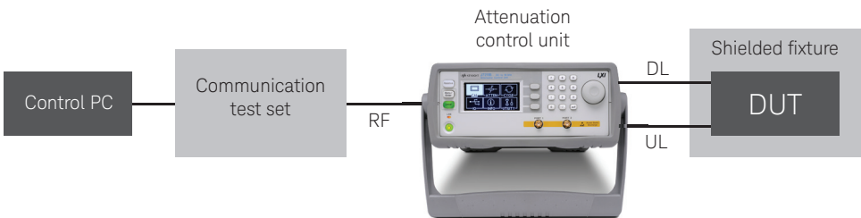
Figure 2. Test setup for mobile receiver sensitivity test using a communication test set
