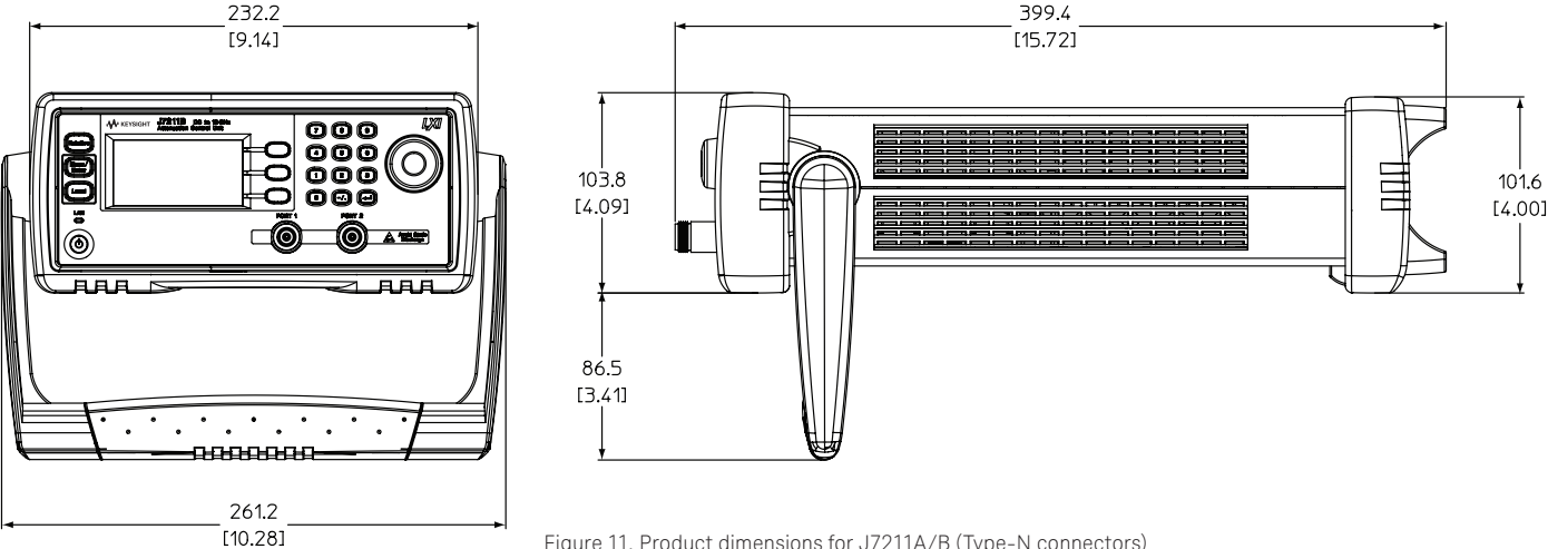
Figure 11. Product dimensions for J7211A/B (Type-N connectors)
