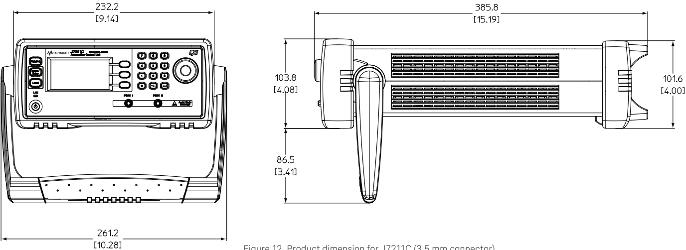
Figure 12. Product dimension for J7211C (3.5 mm connector)
