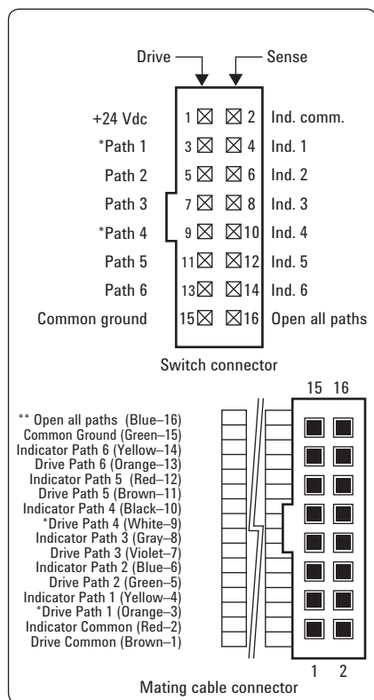
Figure 10. Drive connection diagrams with Option 161
