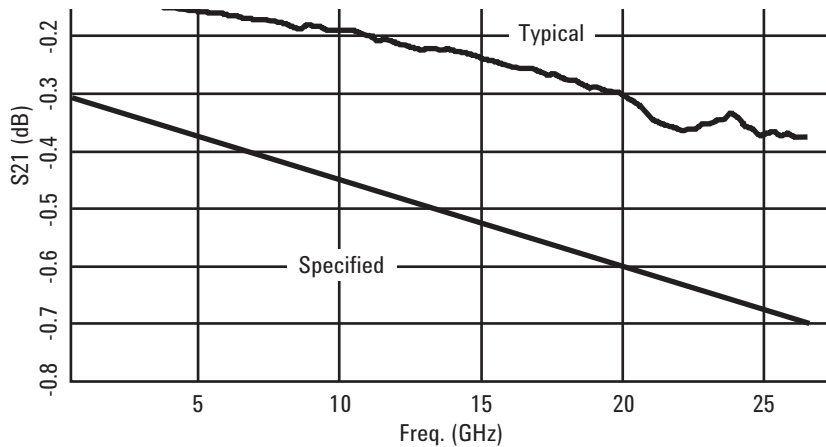
Figure 7. Insertion loss
