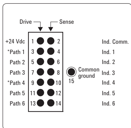
Figure 11. Drive connection diagrams with Option 100
