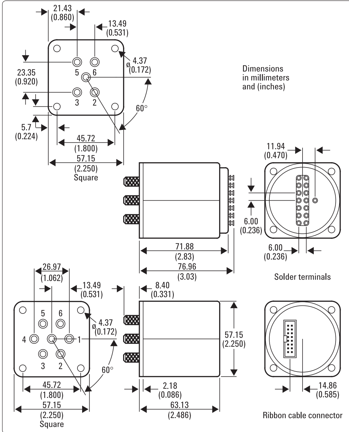
Figure 9. Product outlines
