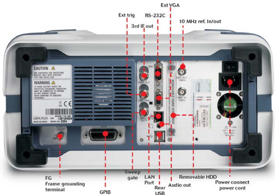
Back of 3250 Series
