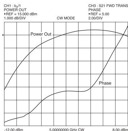
Power Out and Phase performance as a function of Input Power at a CW frequency.
