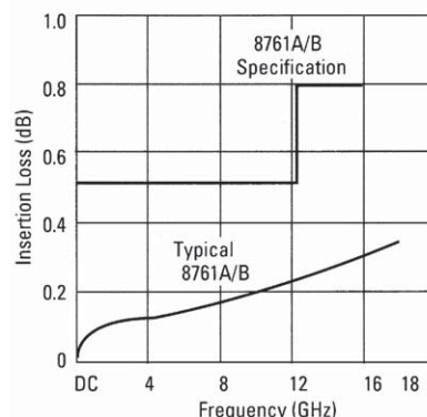
Figure 2. Typical insertion loss
