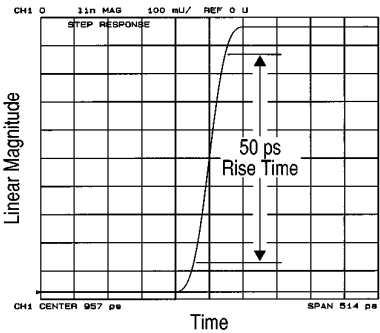
Lightwave step response transmission test (DUT = 21 cm single mode fiber)
