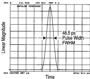
Lightwave impulse response transmission test (DUT = 21 cm single mode fiber)
