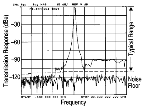
Electrical- to-electrical transmission test (DUT = filter)
