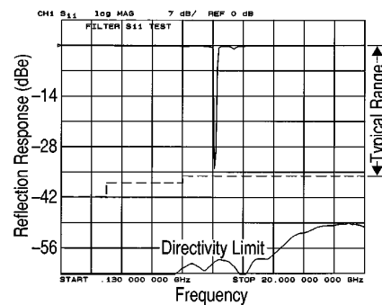
Electrical reflection test (DUT = filter)
