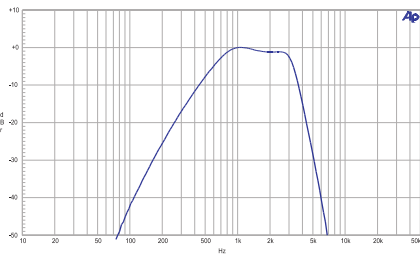
Figure 10. FIL-CMS. C-Message Weighting Filter (ANSI/IEEE 743-1984).
