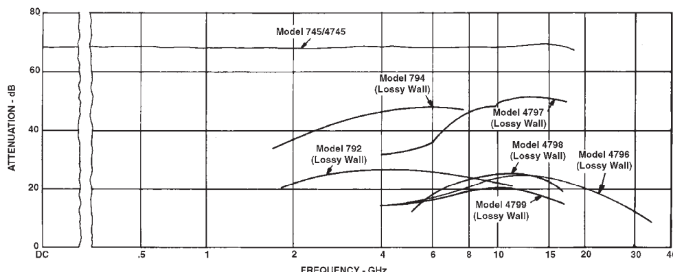
Figure 2. Attenuation vs. Frequency of Variable Attenuators
