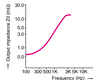
[Fig.-17] Output Impedance Characteristics of PAK35-10A
