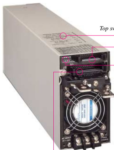
Rear control terminal J2 (Factory-installed option: for connection to PIA4810)
