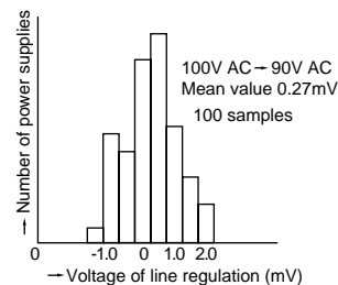
[Fig.-3] Distribution of Line Regulation (CV Characteristics)
